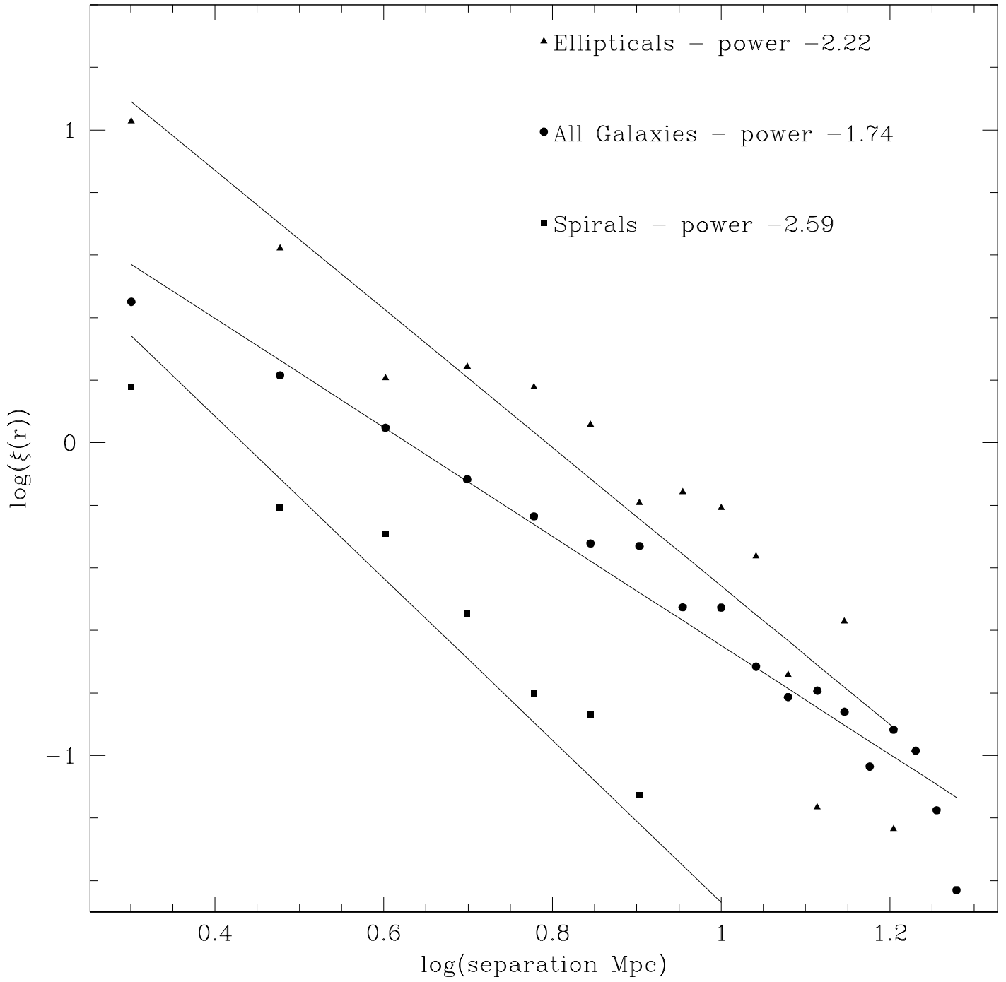
Calculations/Fits of \xi(r) for Galaxy Samples
