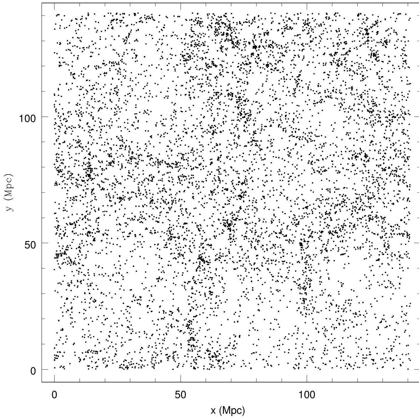
All Galaxies in Data - 8384 galaxies
