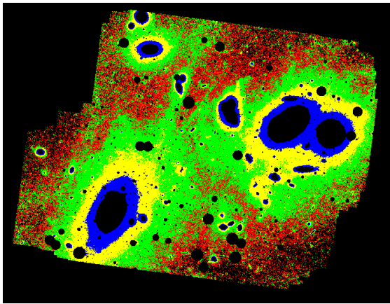
FIG. 2.— Diffuse light in the Virgo cluster, color coded by surface brightness: Blue: \mu_V=25-26 ; Yellow: \mu_V=26-27 ; Green: \mu_V=27-28 ; Red: \mu_V=28-29 . North is up; east is to the left.
