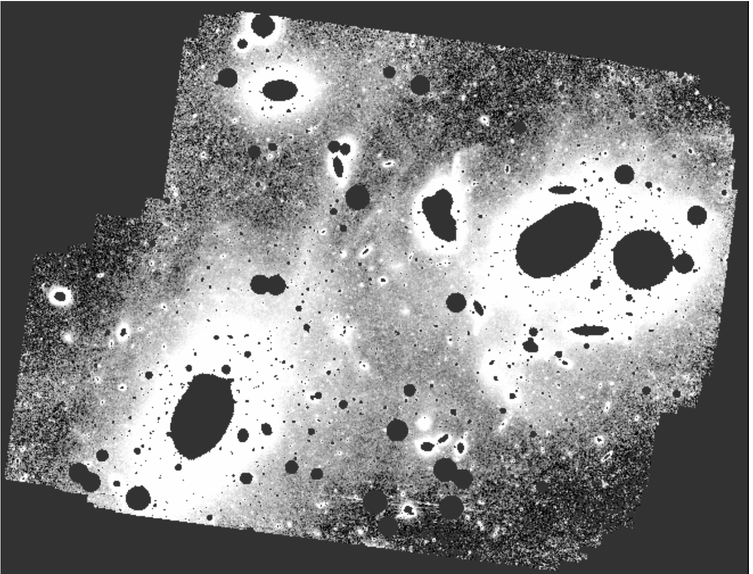
FIG. 1.— Diffuse light in the Virgo cluster core. North is up; east is to the left. The white levels saturate at \mu_V \sim 26.5 , while the faintest features visible have a surface brightness of \mu_V \sim 28.5 .
