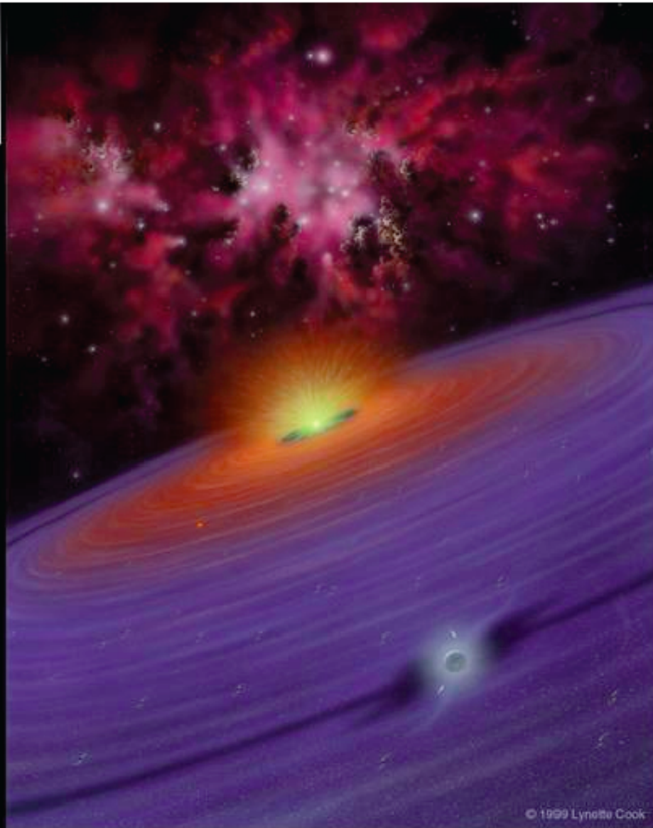
Giant Planets
